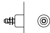
Detail A Earth boss M10
